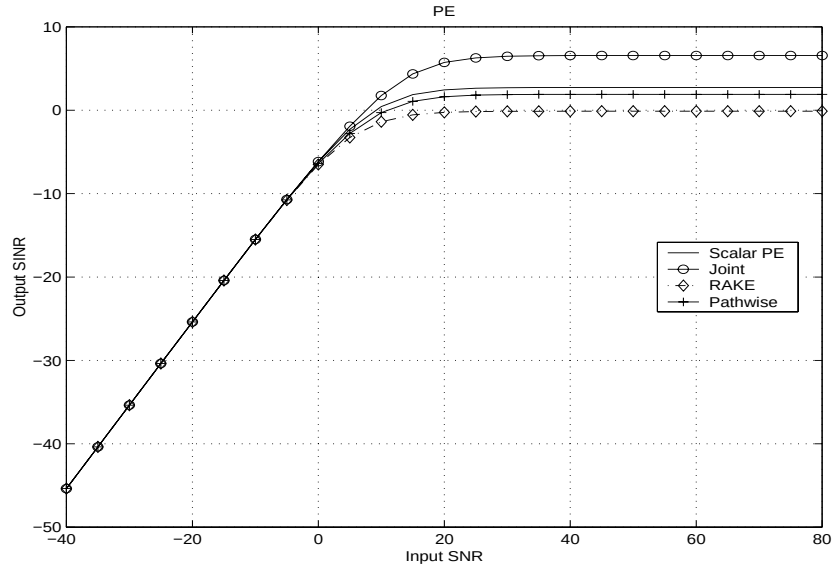
Figure 3.6: Polynomial expansion: L=16 , K=8 , M=1 , unequal power users
