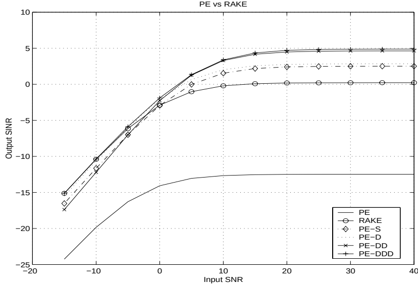
Figure 3.3: Polynomial expansion vs. RAKE: K = 12 , L = 16 , SIR = -10\text{dB}
