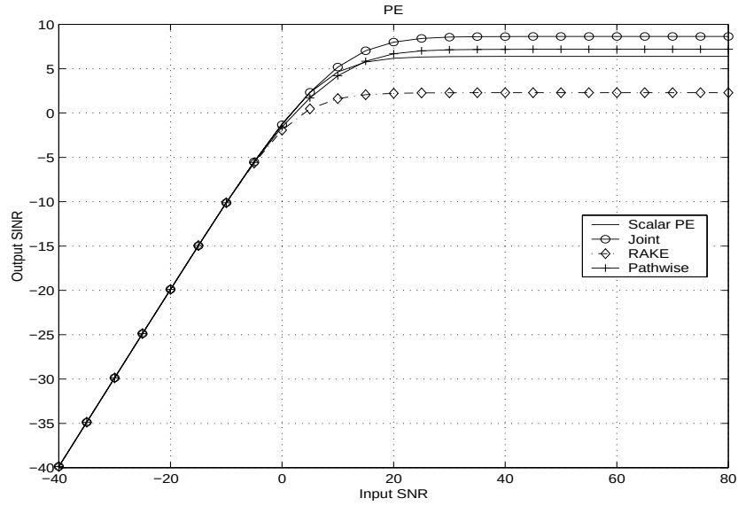
Figure 3.7: Polynomial expansion: L=16 , K=8 , M=2 , equal power users
