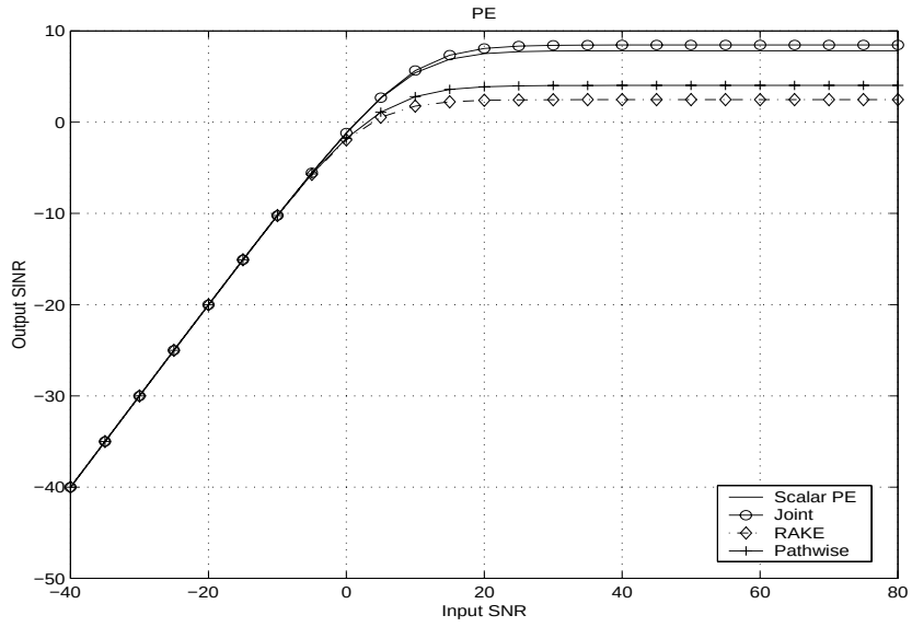
Figure 3.5: Polynomial expansion: L=16 , K=8 , M=1 , equal power users
