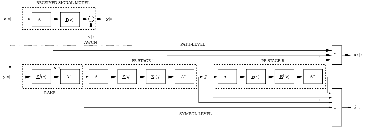
Figure 4.1: Amplitude and symbol estimation suggested by LS results
